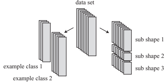
Figure 2. Data vectors in the training set, when the training set is split into subsets one obtains a mixture model (left part of figure); when the vectors are split one obtains the model presented in this paper (right part of figure).
