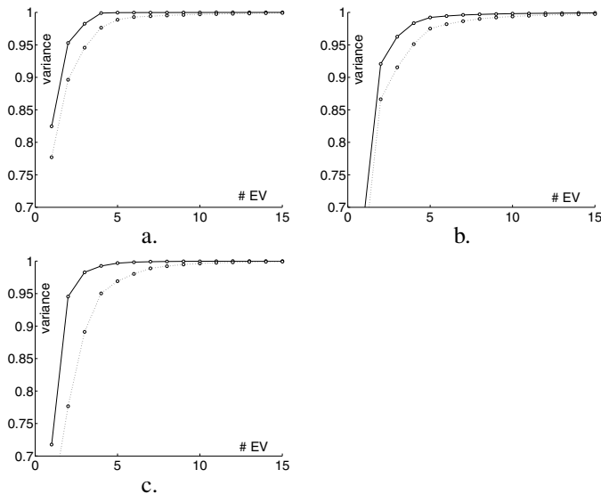
Figure 8. Captured variance for a. rectangle data b. bone data and c. hand contour data, the x-axis corresponds to the number of eigenvectors, single model dashed-line sub-shape model solid line.
