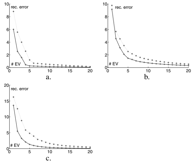
Figure 9. Reconstruction error for a. rectangle data b. bone data and c. hand contour data, the x-axis corresponds to the number of eigenvectors, single model dashed-line sub-shape model solid line.
